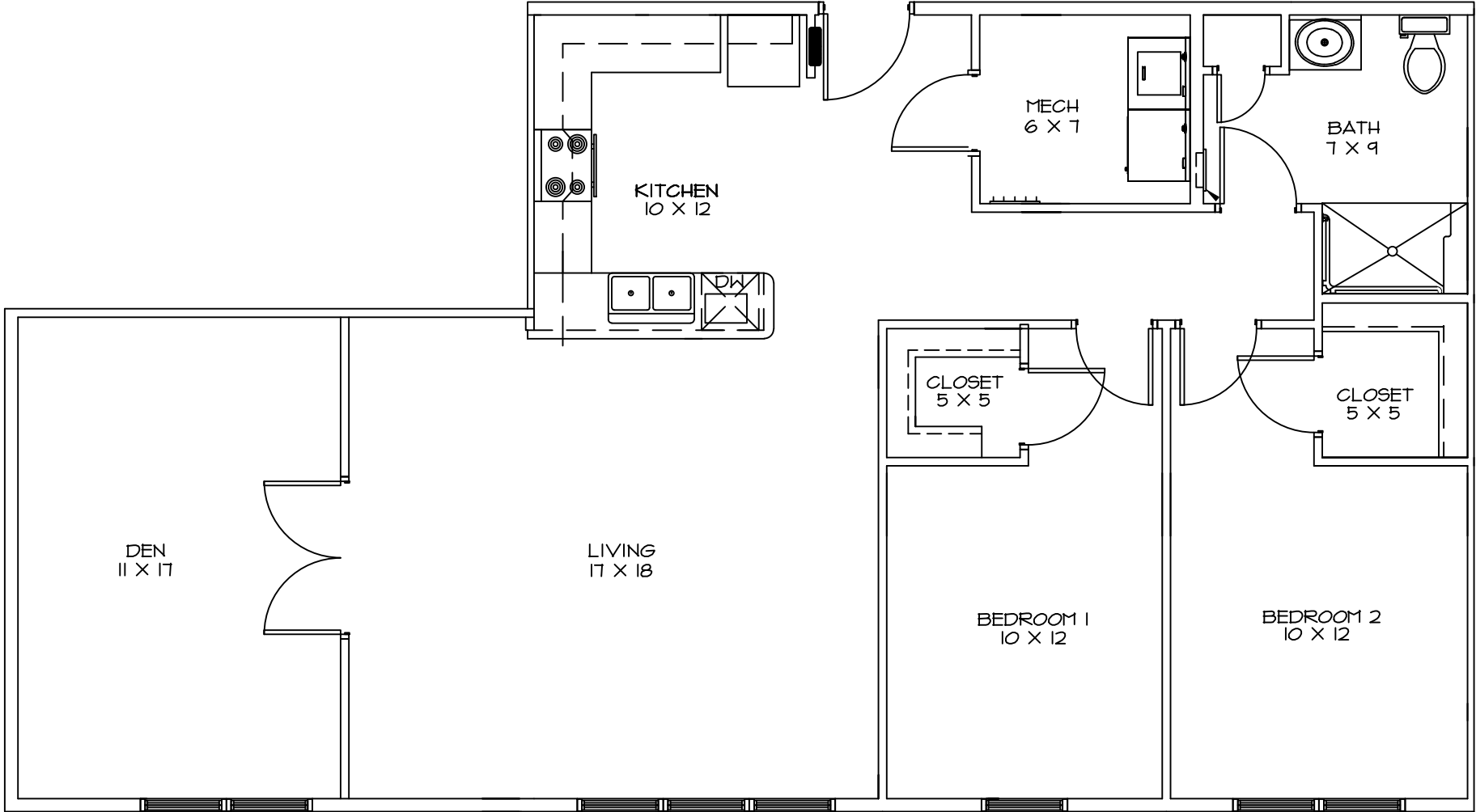
DELUX TWO BEDROOM UNIT-TYPE (ACCESSIBLE) "DD" NEAT RENTABLE AREA = 1,224 SQ. FT. NET/1,275 SQ. FT. GROSS
