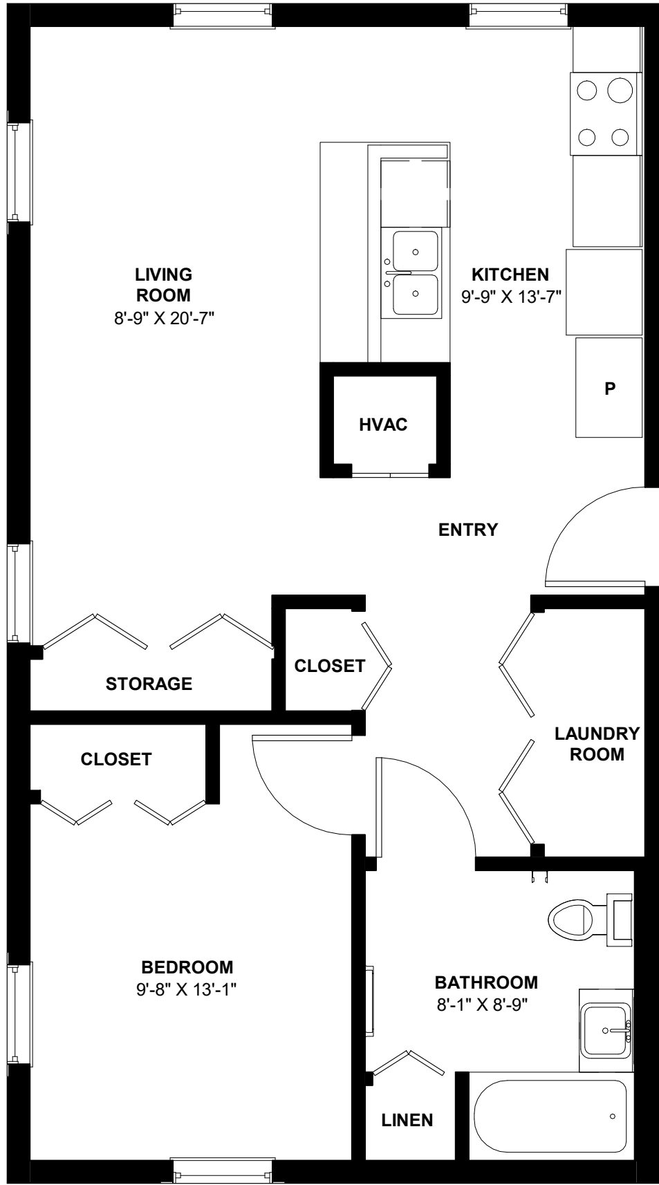
UNIT 101 - TYPE ADAPTABLE
